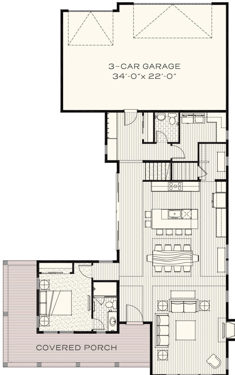
FIRST FLOOR
